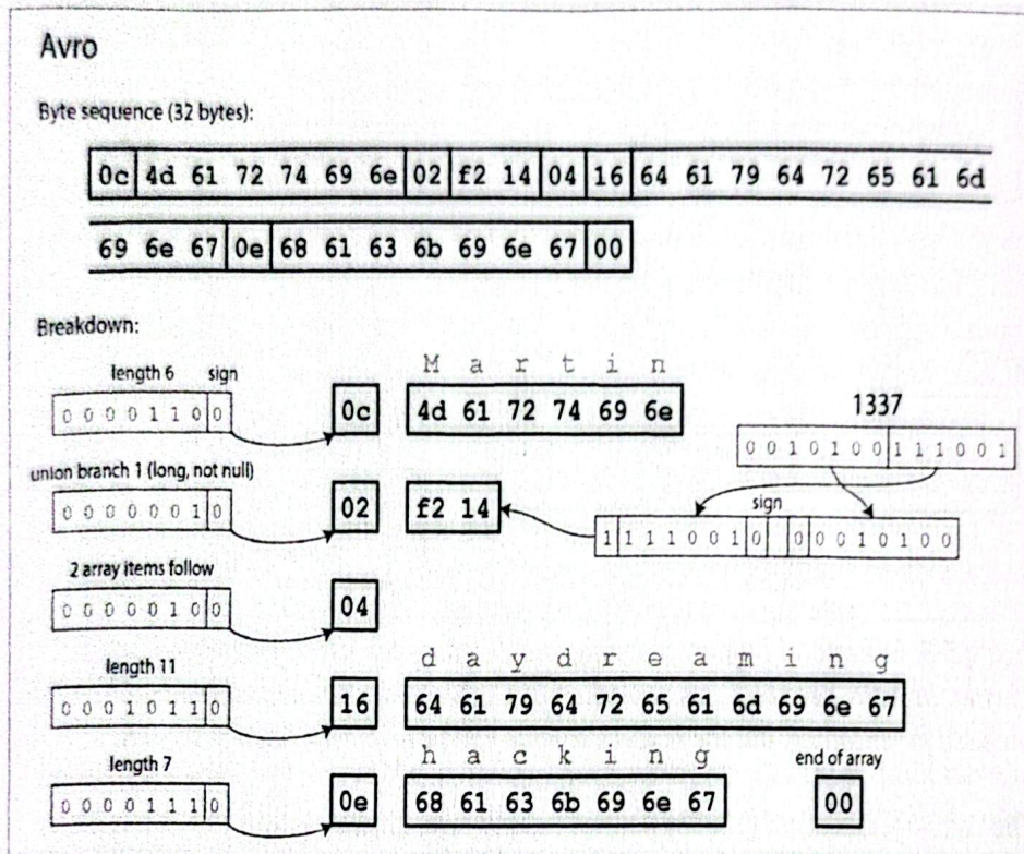
Figure 5-4. Our record encoded using Avro
